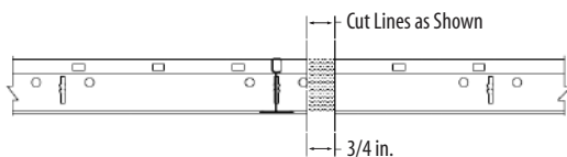
1 - On Intersection - On Joint Cut
