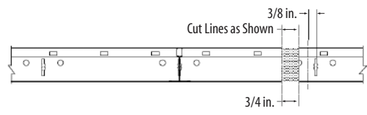
3 - Off Intersection - Off Joint Cut
